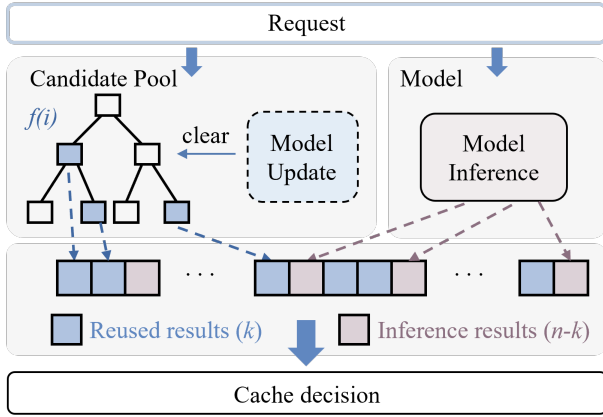
Fig. 3. The adaptive inference reusing process of LBSC^+ .
