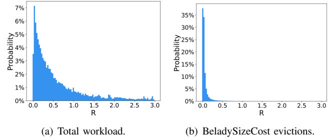
Fig. 4. Distribution of \mathcal{R} between the total workload and BeladySizeCost evictions.
