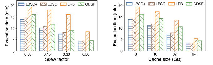
Fig. 12. End-to-end execution time comparison among LBSC^+ , LBSC, LRB, and GDSF in OceanBase.
